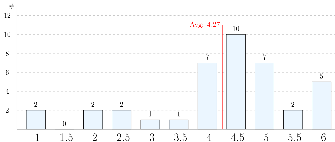
Distribution of Grades: First Exam Fall 2017
